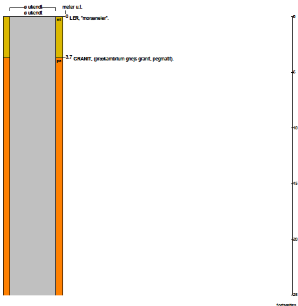
Figure 38. Geological log from the borehole DGU NO. 244.554: Upper part of the 60 m deep raw material borehole. (From the GEUS Jupiter database).
