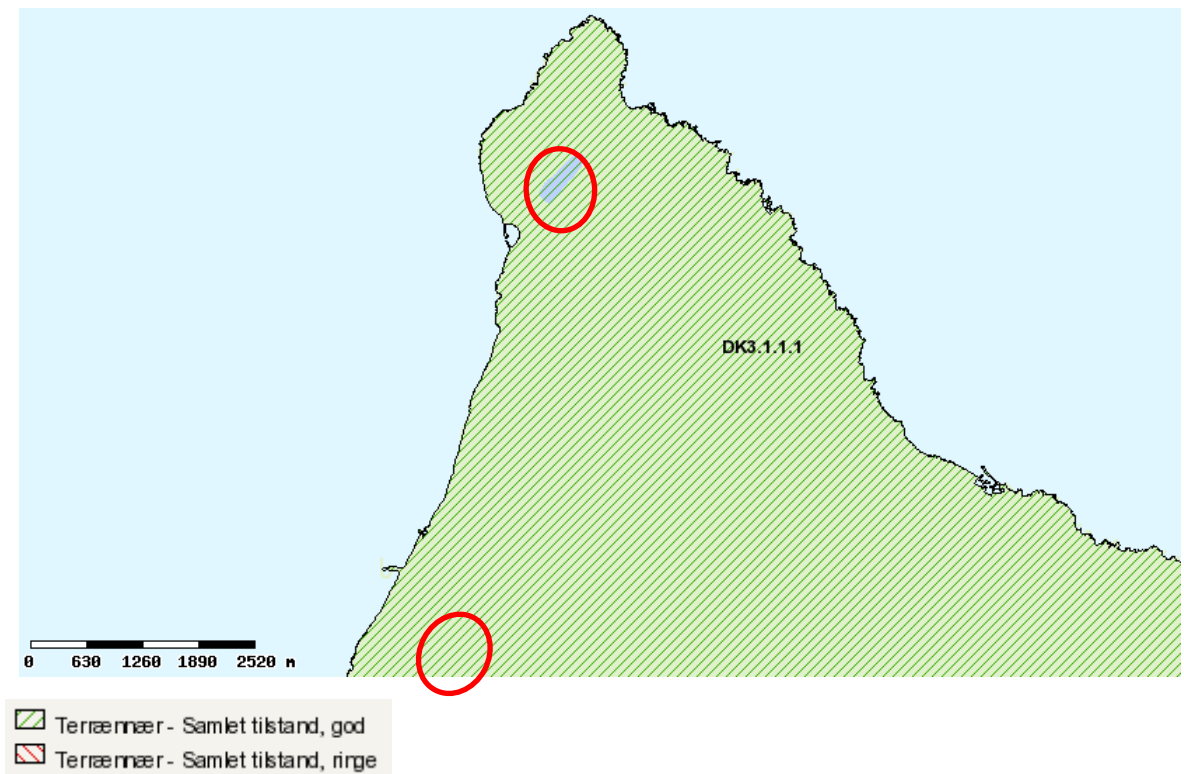
Figure 53. Shallow (or terrain near) groundwater body DK3.1.1.1. Red circle show the location of the two suggested locations of Area 2 in the Granite quarries in Hammeren or Vang. (From Miljøministeriet, 2010.)
